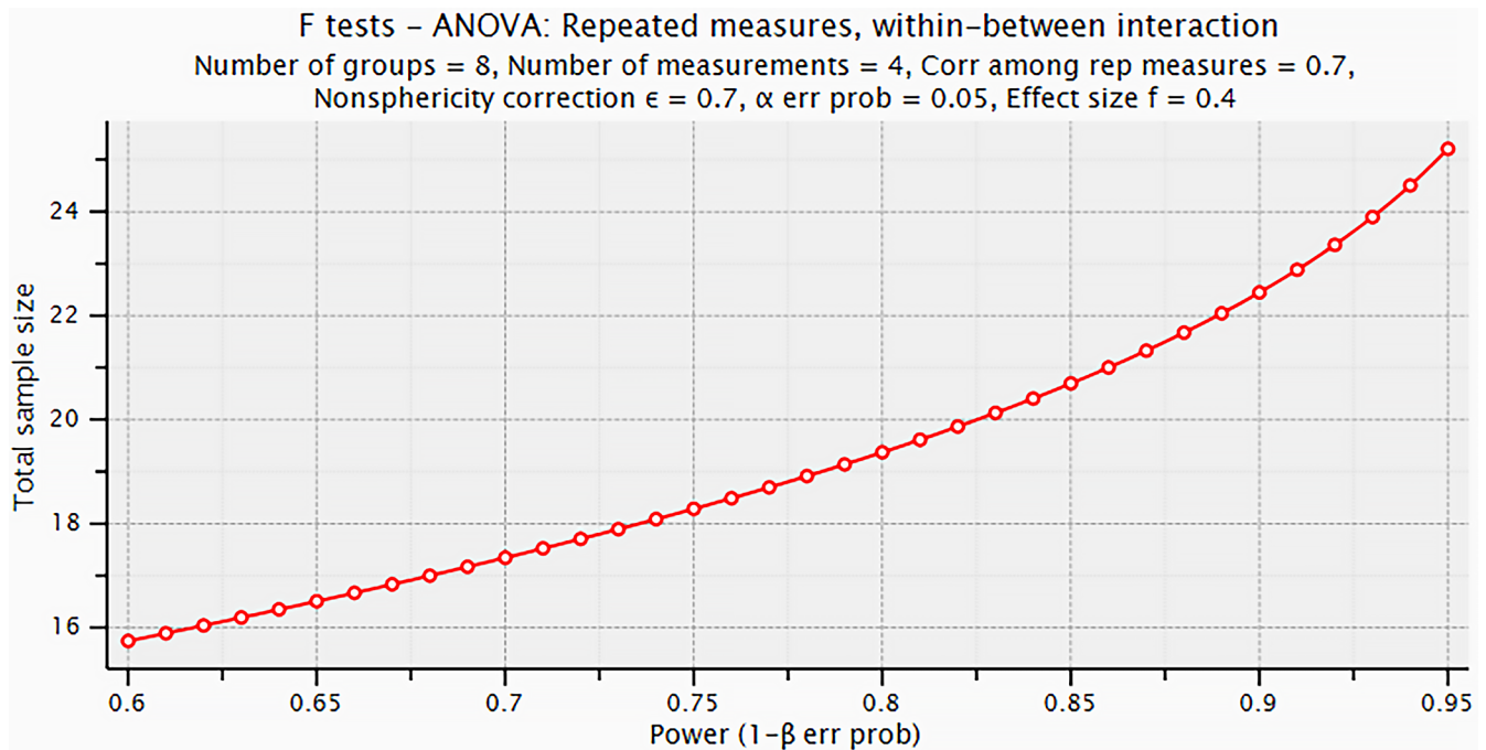
Fig. 3. Relationship between required sample size and statistical power
